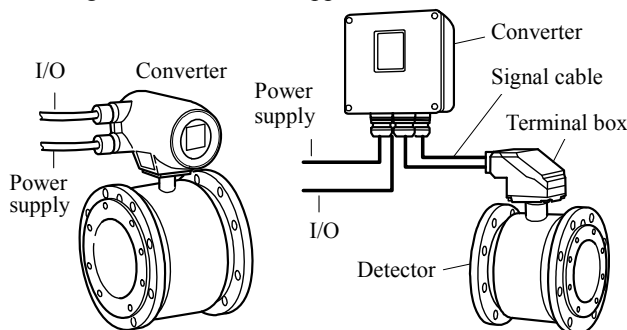
Combined type LF430/LF600 LF434/LF600F
