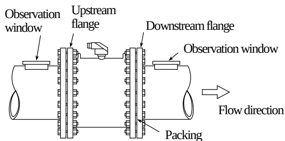
Figure 6. Flange Connection
