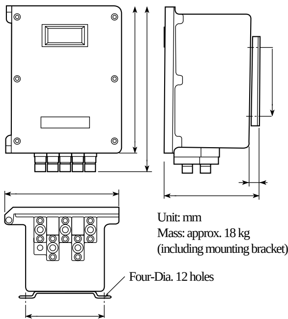
Figure 5. Converter Dimensions
