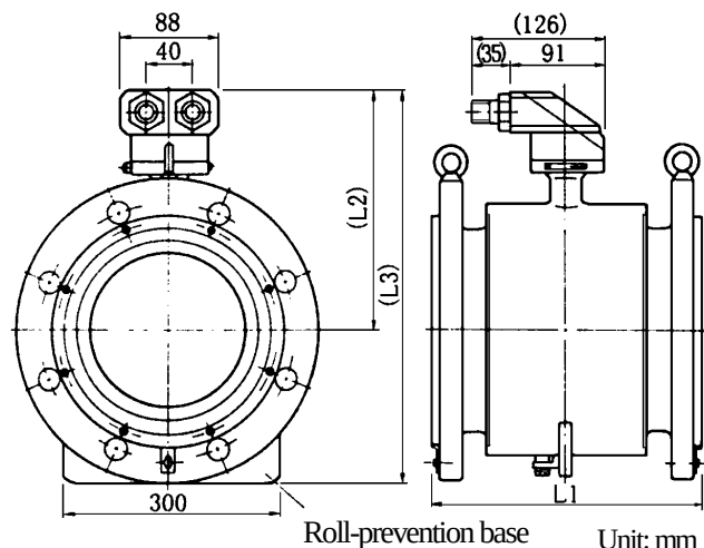
Figure 4. Detector Dimensions for Meter Sizes 250 mm (10'') to 600 mm (24'')
